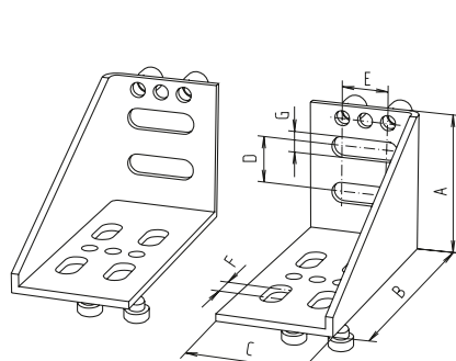
Steel angle bracket 60x120, 1 brace left or right
