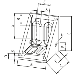
Angle bracket F-60x60 Die-cast zinc
