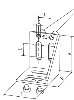
Steel angle bracket 60
