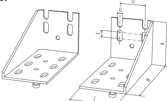
Steel angle bracket 60x160, 1 brace left or right
