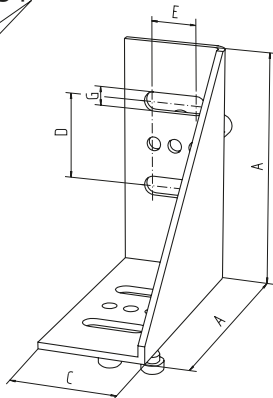
Steel angle bracket 60 / 60x120
